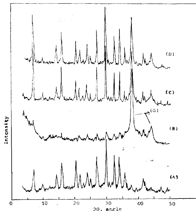
Figure 1. X-Ray diffraction of Ag_{12} -A: (A) Ag_{12} -A dehydrated at 300°C under 10^{-4} mmHg; (B) Dehydrated Ag_{12} -A treated by flowing H_2 gas; (C) Hydrogenated Ag_{12} -A treated by flowing O_2 at 200°C; (D) Hydrogenated Ag_{12} -A treated by flowing O_2 at 100°C; (G) These peaks are (111) and (200) diffractions of silver metal.
