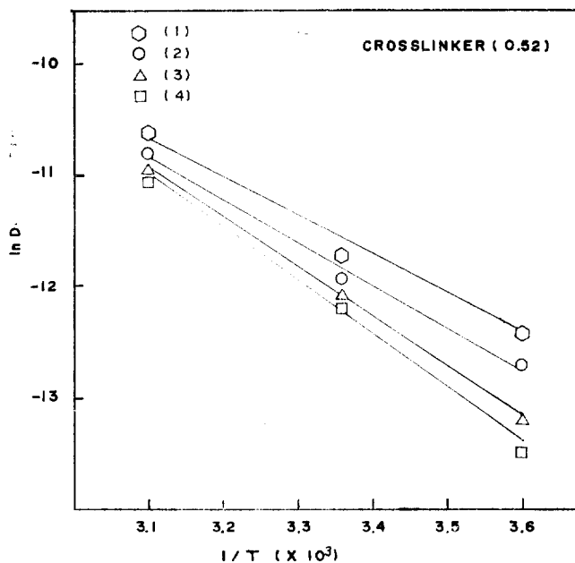
Figure 5. The plot of \ln D versus 1/T for copolymer hydrogel membranes with 0.52 mole % crosslinker.
