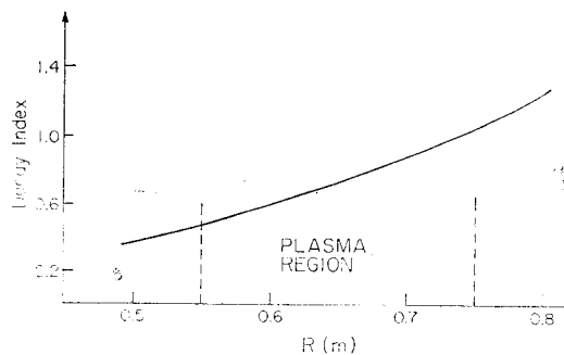
Fig. 7. Decay Index along the Radial Direction at z=0 Plane.
