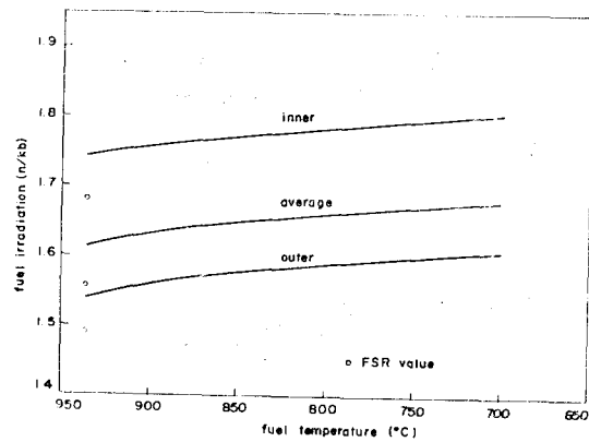
Fig. 7. Average Discharge Irradiation v.s. Fuel Temperature
