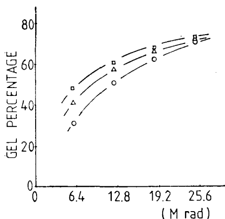
Fig. 8. Effect of TMPTM concentration and radiation dosage on gel fraction of PE-5031.
