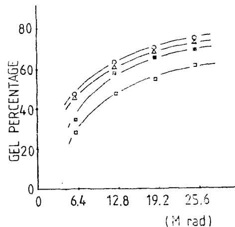
Fig. 3. Effect of Santonox R concentration on gel fraction of PE-301.
