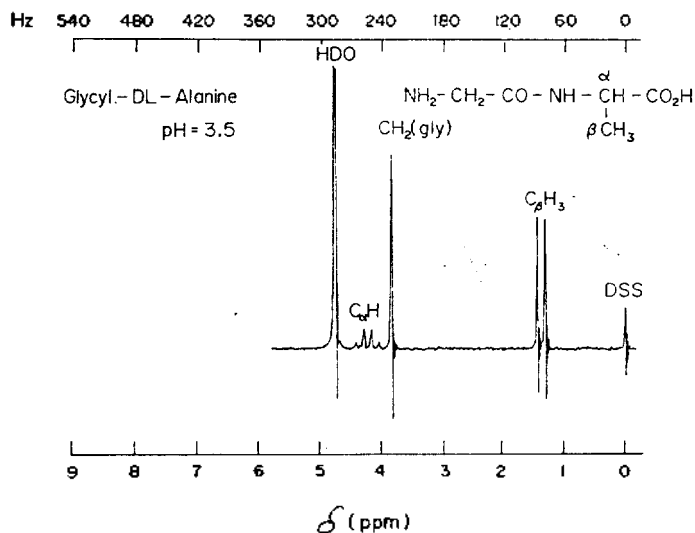
Fig. 2. Proton magnetic resonance spectra of solutions of glycyl- DL -alanine in D_2O taken at a spectrometer frequency of 60 MHz at pH 3.5.
