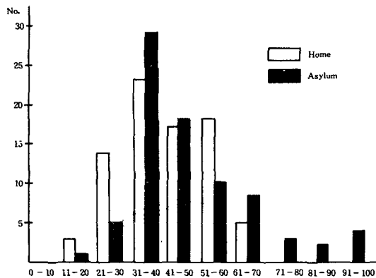
Fig 1. CMI Scores
