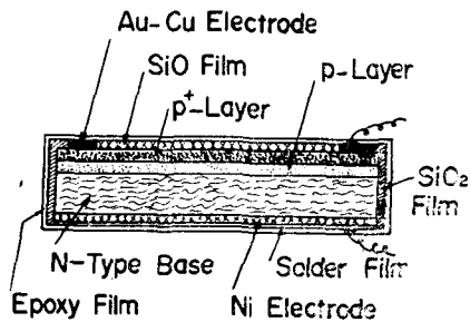
Fig. 5. Sectional view of the fabricated p^+ - p - n type silicon solar cell
