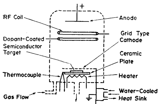
Fig. 3. Schematic illustration of the GDH-Implanter
