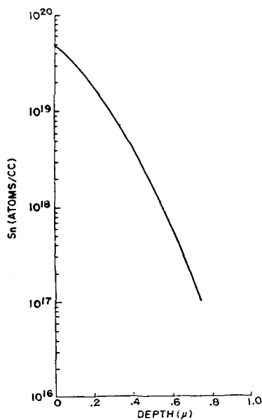
Fig. 6. Sn profile in presence of B diffused at 1200^{\circ}C , 60 min (after Yeh and Joshi)
