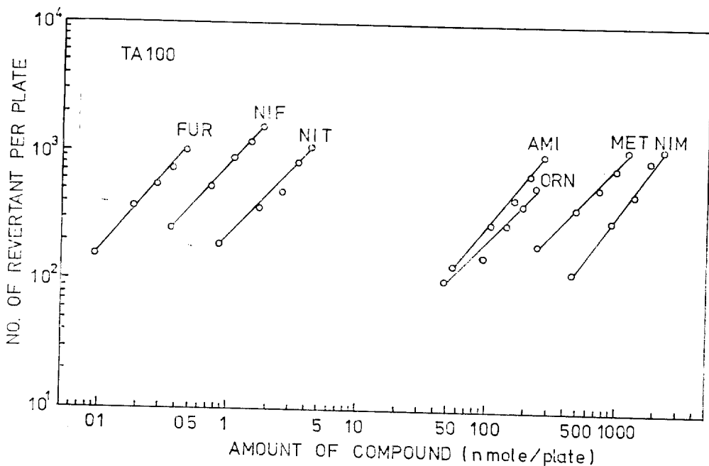
Fig. 2 Dose response of mutagenic trichomonacides
