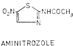
Fig. 1 Chemical structure of mutagenic trichomonacides
