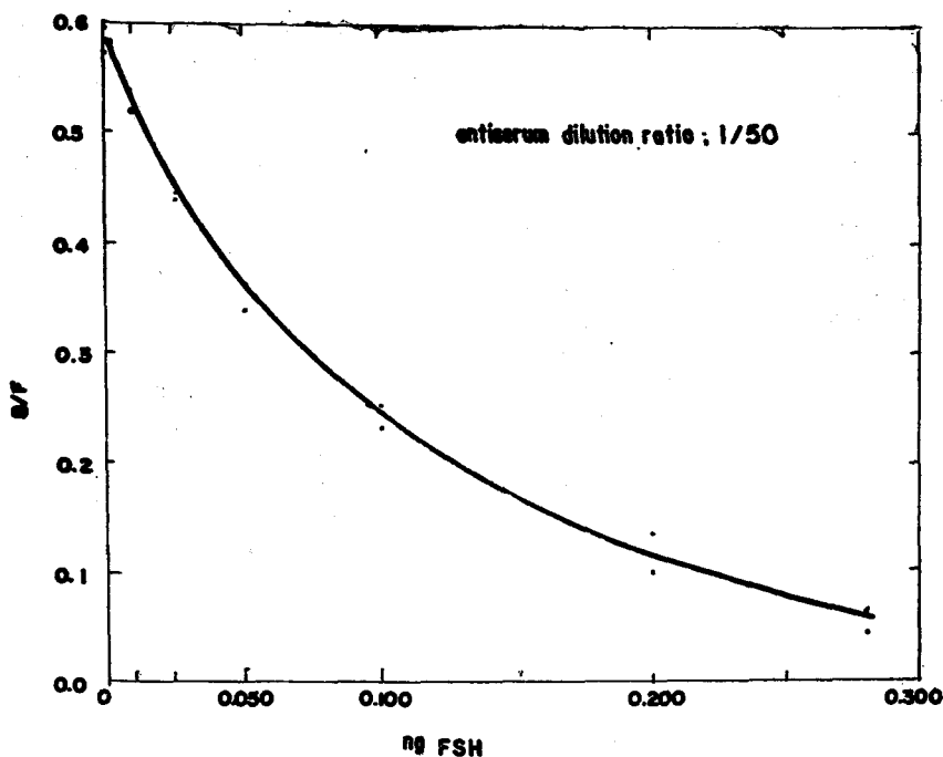
Fig. 7. Standard dose response curve.
