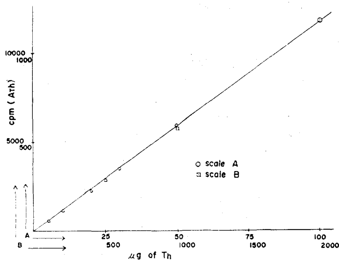
Fig. 3. Calibration curve of 1~1000 \mu g standard thorium samples (Irrad. time 1min.; power level 2MW; counted for 1min. after 20 sec delay)
