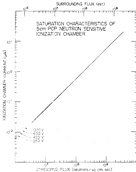
Fig. 9. Saturation characteristics for the PCP chamber in the streaming flux level of 10^9 nv.
