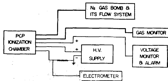
Fig. 6. Block diagram of the whole measuring system of the PCP chamber.
