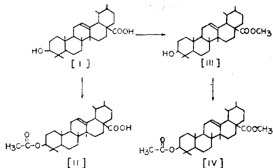
Fig. 1. The scheme of separation and purification of sapogenin.
