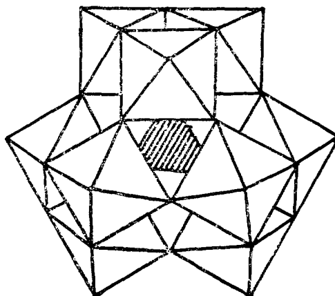
Fig. 1. Polyhedral model of the Keggin-structure anion
