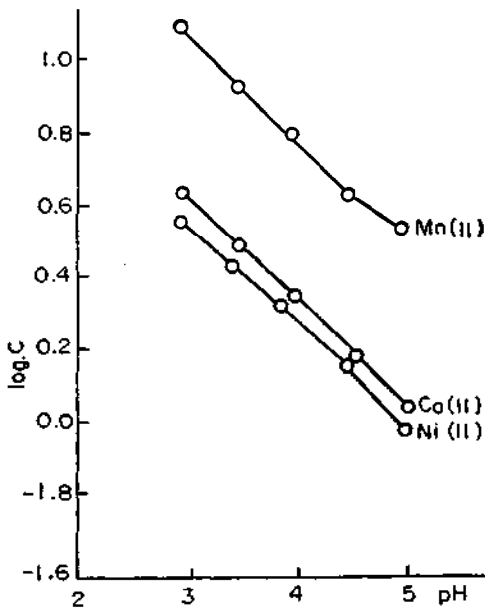
Fig. 2. Plots of log C vs. pH Resin: Dowex 50 w × 12 (100~200 mesh) Eluent: 0.7 M NaCl + 0.05 M Na 2 C 2 O 4
