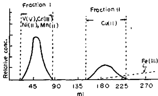
Fig. 4. Elution Curves of cation in the sample Resin; Dowex 1 × 8 (100~200 mesh) Column; 15 cm × 3.14 cm 2 Eluents; 4.0 M HCl
