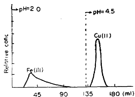
Fig 6. Elution Curves of Cations [Cu(II), Fe(III)] in fraction II Resin; Dowex 50w × 12(100~200 mesh) Column; 10 cm × 3.14 cm 2 Eluent; 0.6 M NaCl + 0.1 M Na-tartrate
