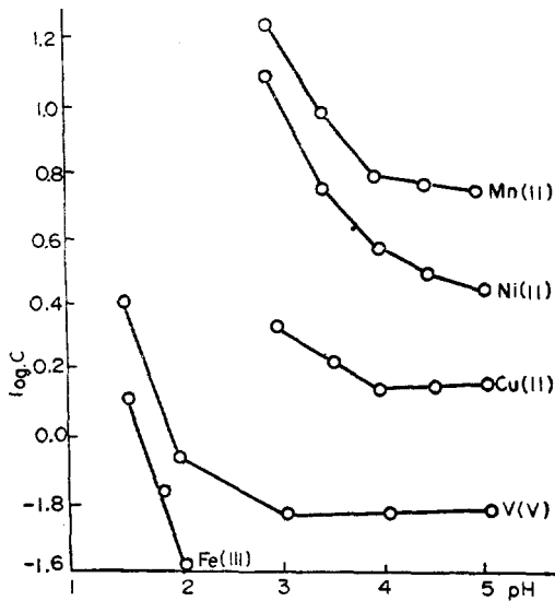
Fig. 1. Plots of log C vs. pH Resin: Dowex 50 w × 12 (100~200 mesh) Eluent: 0.6 M NaCl + 0.1 M Na-tartrate
