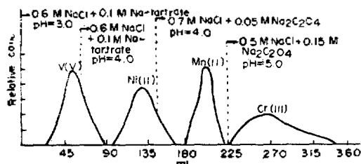
Fig 5. Elution Curves fo Cations [V(V), Ni(II), Mn(II); Cr(III)] in fraction I Resin; Dowex 50w × 12(100~200 mesh) Column; 10 cm × 3.14 cm 2
