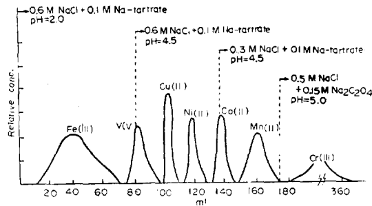
Fig. 3. Elution Curves of Synthetic mixture Resin; Dowex 50 w × 12 (100~200 mesh) Column; 35 cm × 3.14 cm 2
