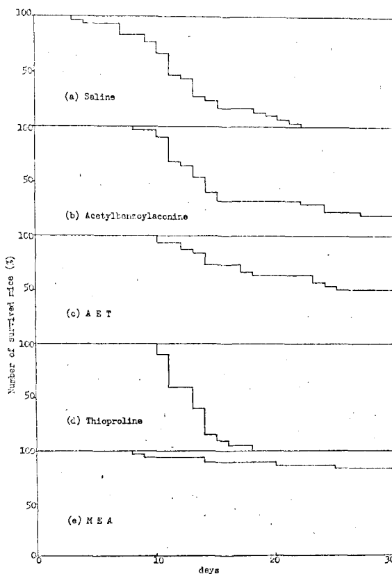
Fig. 2. Survival curves after 800 rad gamma-ray irradiation.
