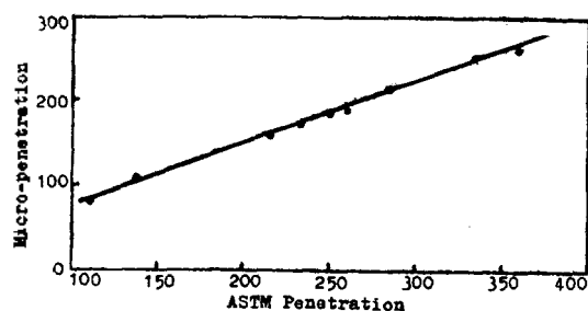
Fig. 2 ASTM Penetration vs Micro-Penetration
