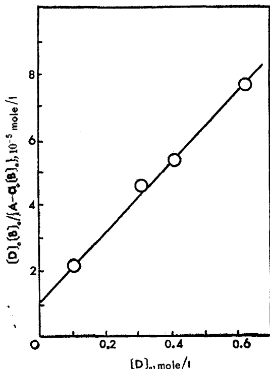
Fig. 1. — Plots of [D]_0[B]_0/[A-a_0(B)_0] versus [D]_0 of the o -toluidine-iodine system at 19°C.
