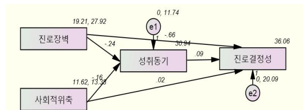
Fig. 1. Path analysis of structural model
