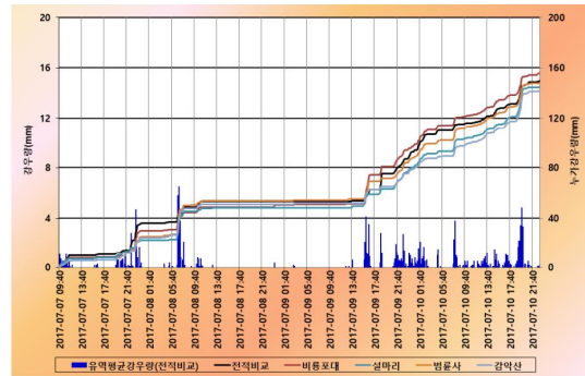
(2) 10분 누가강우량곡선(2017.07.07~07.10)
