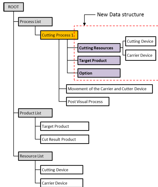
Fig. 1. Data Structure.
