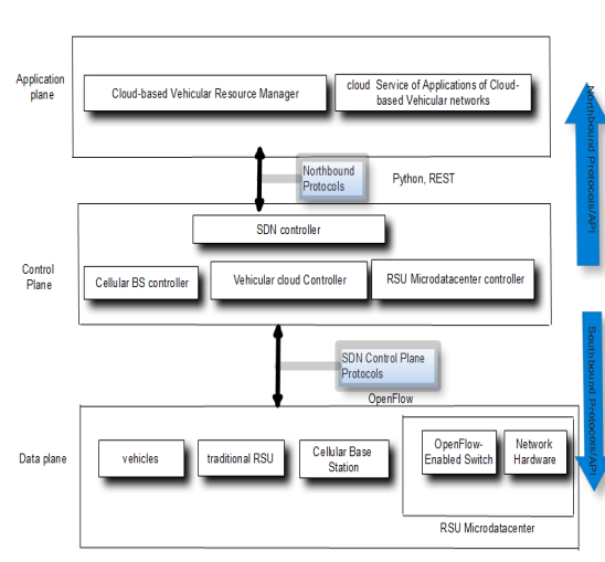
그림 2. Logical structures of the SDCVN includes data and control planes.
