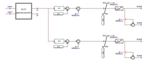
Figure 3 Generating MMC valve control command
