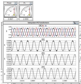
Figure 4 3-phase balanced current waveforms
