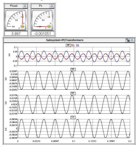
Figure 5 3-phase unbalanced current waveforms
