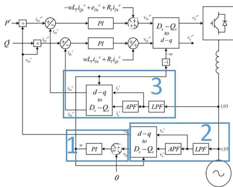
Figure 2 Control block diagram
