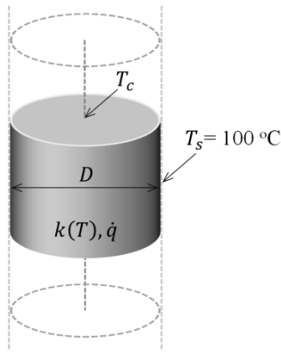
Fig. 1. Scheme of centerline temperature ( T_c ) calculation ( T_s : surface temperature, k : thermal conductivity, q : heat generation, D : diameter).
