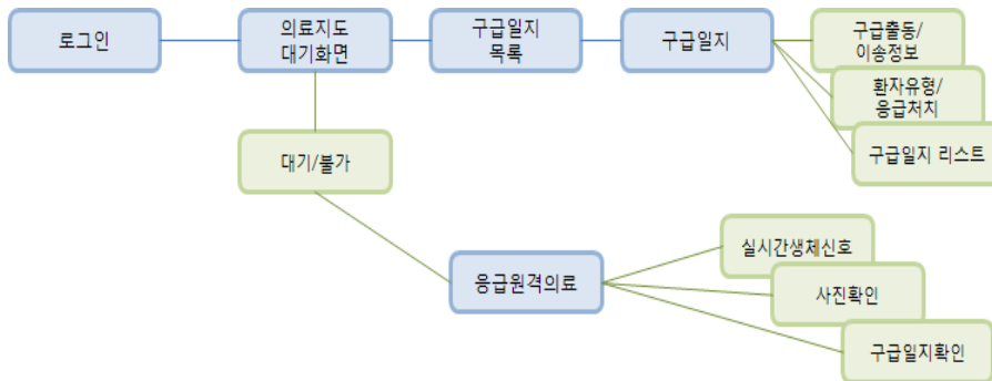
Fig. 3 The UI Structure of remote medical treatment support application.
