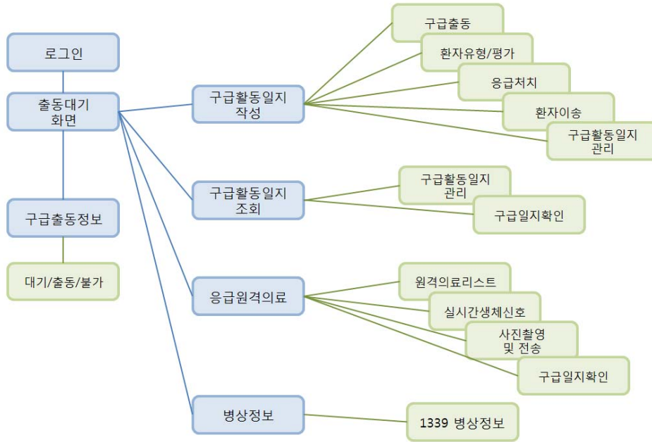
Fig. 2 The UI Structure of paramedic support application.
