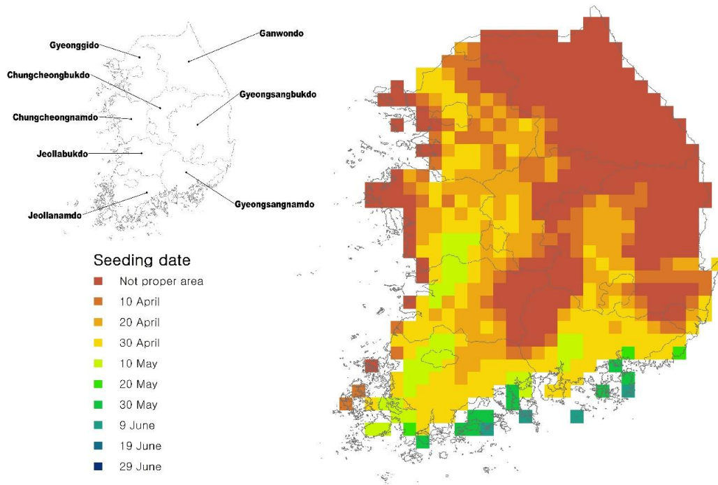
Fig. 1. The optimal seeding dates in the 1990s, which were determined using regional climate model data as inputs to the ORYZA2000 model. The regional climate data at a spatial resolution of 12.5 km were obtained using the HadGEM3-RA model through dynamic downscaling of global climate scenario data.
