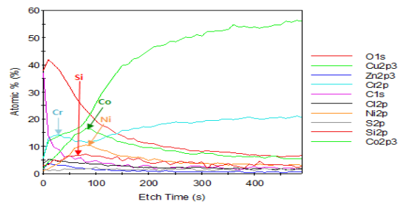
Fig. 2. Results of depth profile Cu carrier film
