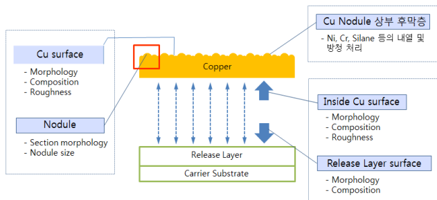
Fig. 1. Schematic of copper carrier film
