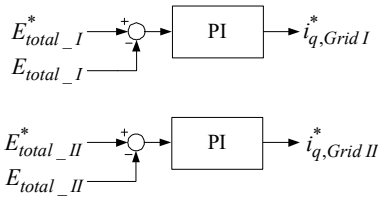
Figure 3. Proposed total capacitor energy controller
