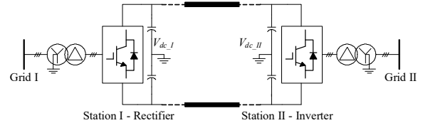
Figure 1. Conceptual structure of the transmission system by the conventional method.
