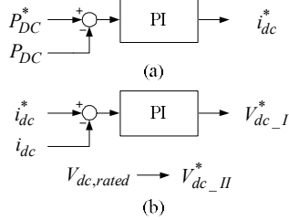
Figure 4. Proposed power flow controller. (a) Transmission line current generator. (b) Transmission line regulator.
