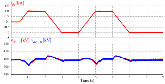
Figure 5. Transmission line current and voltages under the conventional control strategy during power flow variation.
