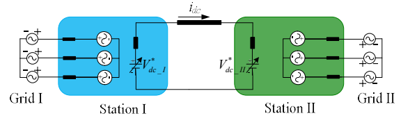
Figure 2. Conceptual structure of the transmission system by the proposed method.
