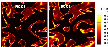
Fig. 5 Contours of HRR at \tau_{ig}^0 under RCCI and SCCI conditions ( r' = 0.44 and T' = 15 K).
