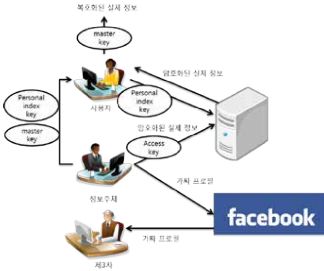
3 FaceCloak Architecture
