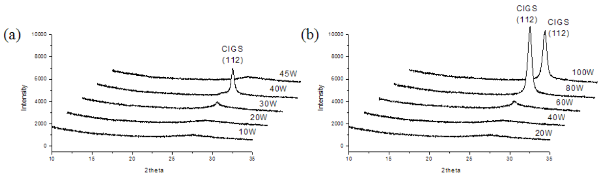
Fig. XRD patterns of CIGS(1 \mu m) films deposited at various DC and RF power ;
