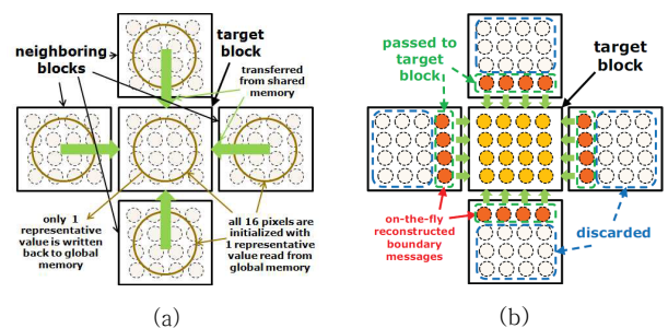
Fig 1. Proposed algorithm. (a) Data transfer in the proposed algorithm. (b) On-the-fly boundary message reconstruction
