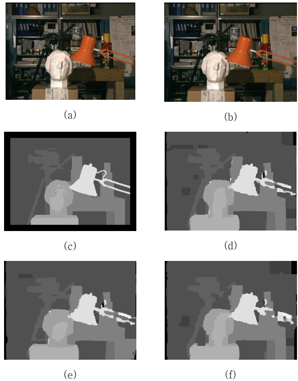
Fig 3. Depth map obtained for Tsukuba testset. (a) Left image. (b) Right image. (c) Ground truth. (d) Hierarchical BP-M. (e) Tile-based BP. (f) Proposed algorithm.
