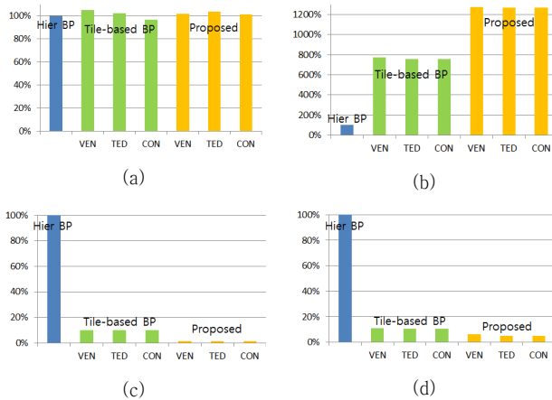
Fig 2. Comparison between hierarchical BP-M, tile based BP, and the proposed method on Tsukuba, Venus, Teddy, Cones image. The block size 8x8. (a) Minimized energy. (b) Number of message computation. (c) Consumed global memory. (d) Global↔local data transaction.
