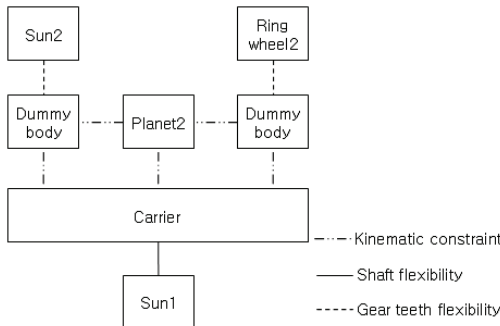
Fig. 3 Model of the second planetary gear
