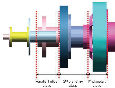
Fig. 2 Model of the gear box
