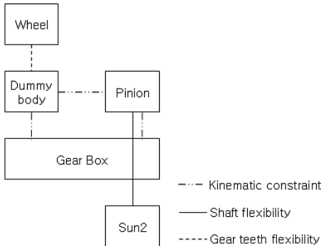
Fig. 4 Model of the parallel transmission
