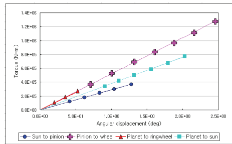
Fig. 5 Torsional stiffness
