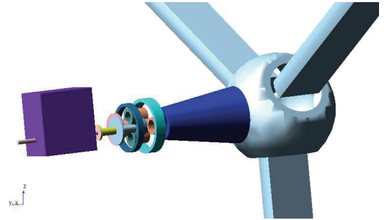
Fig. 1 Model of the complete DT
