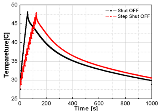
Fig. 11 Temperature distribution along time
