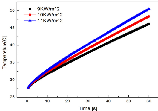
Fig. 12 Temperature distribution along heat source
