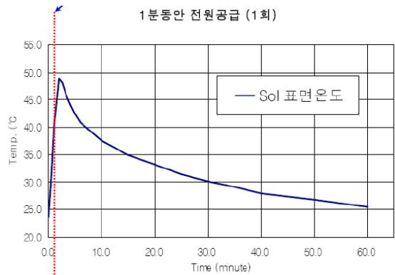
Fig. 6 Temperature distribution of Solenoid(shut-off)
