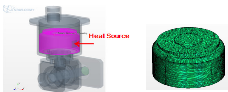
Fig. 3 Thermal Model and Grid
