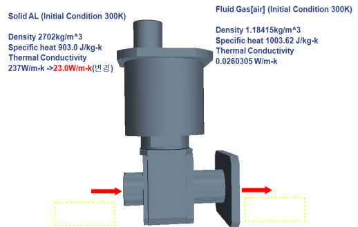
Fig. 4 Boundary Condition
