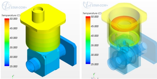
Fig. 9 3-D Temperature distribution at Shut-off
