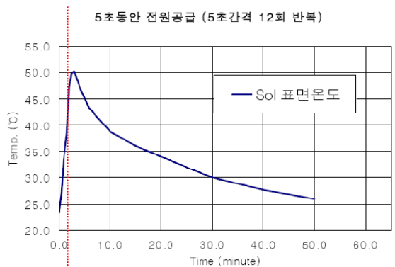
Fig. 7 Temperature distribution of Solenoid(step shut-off)
