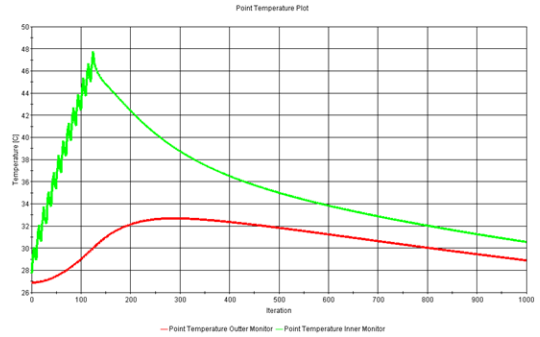
Fig. 10 Temperature distribution at step shut-off
