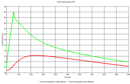
Fig. 8 Temperature distribution at Shut-off
