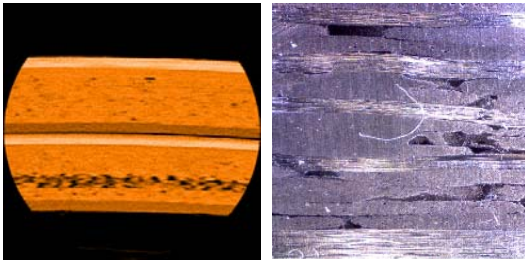
Fig. 8 Image of the Computed Tomography and the Video Microscope about Defect Specimen of the Composite Motor Case
