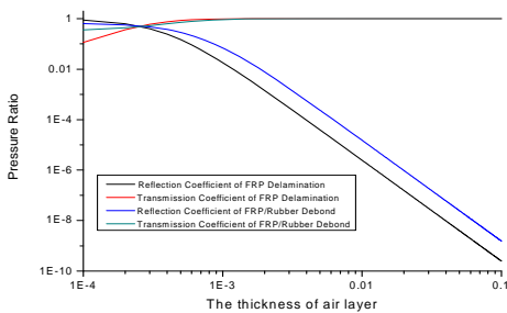
Fig 9. Expectation of Detectable Debonding Width about the FRP Delamination and FRP/Rubber Disbond Interface
