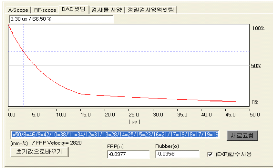
Fig. 5 Distance Amplitude Correction Curve Of Composite Motor Case
