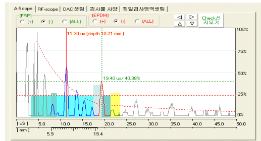
Fig. 4 Adjustment of Defect Detection Level
