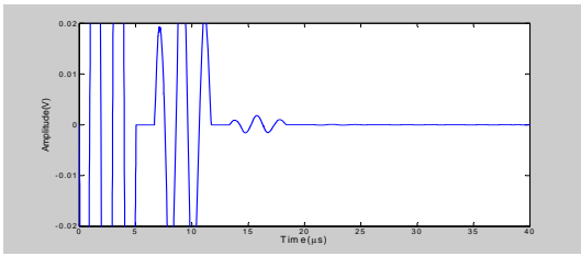
(a) FRP Delamination
