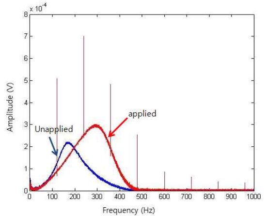
Fig. 7 Frequency Response for MR Elastomer(10mm, Horizontal Magnetized Direction)
