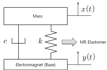
Fig. 6 Modeling of System
