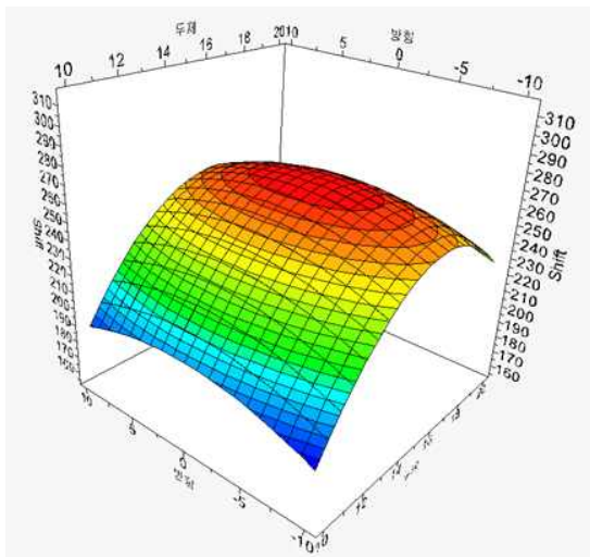
Fig. 8 Response Surface Model
