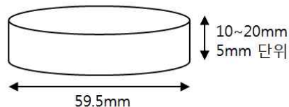
Fig. 1 MR Elastomer Dimension
