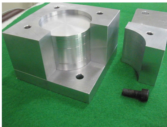
Fig. 2 Mold for MR Elastomer fabrication
