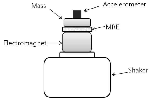
Fig. 5 Diagram of System for MR Elastomer Vibration Test
