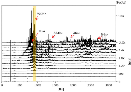
Fig. 4 Waterfall plot for noise of the reducer
