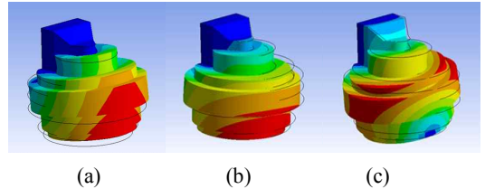
Fig. 8 Mode shapes of the reducer: (a)vertical bending mode, (b)horizontal bending mode, (c)torsional mode
