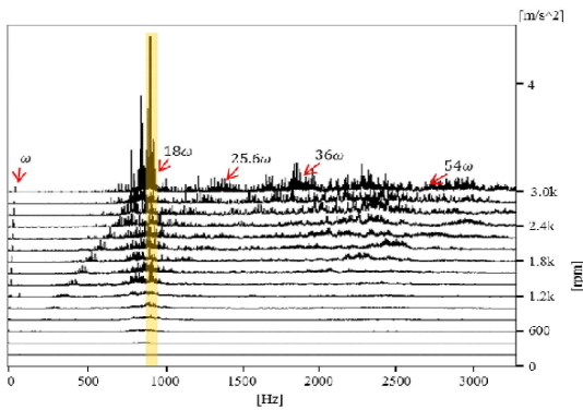
Fig. 5 Waterfall plot for vibration of the reducer
