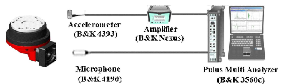
Fig. 3 Experimental setup for signal analysis
