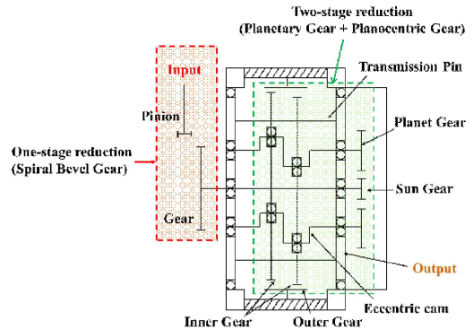
Fig. 2 Basic configuration of the reducer
