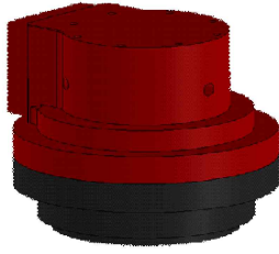
Fig. 9 Structural modification for the housing of the reducer
