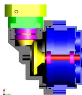
Fig. 1 The reducer designed right angle
