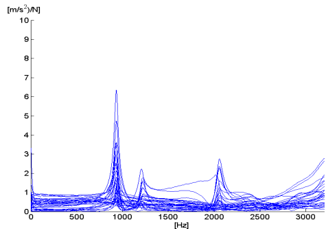
Fig. 7 Frequency response functions of the reducer
