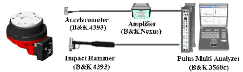
Fig. 6 Experimental setup for system analysis
