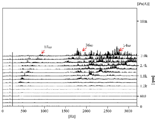
Fig. 10 Waterfall plot for noise of the modified reducer
