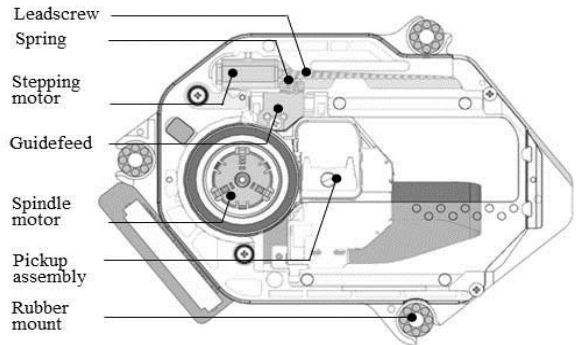
Fig. 1 Structure of Slot-type Optical Disk Drive
