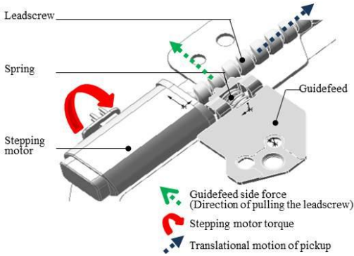
Fig. 2 Structure of Guidefeeding System
