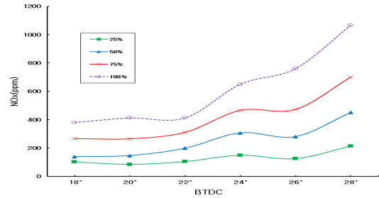
Figure 4. NOx emission characteristics at various fuel injection timing
