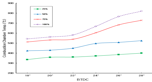
Figure 2. Combustion chamber temperature at various fuel injection timing
