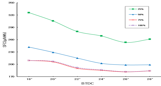
Figure 1. Specific fuel consumption at various fuel injection timing
