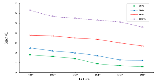
Figure 6. Soot emission characteristics at various fuel injection timing
