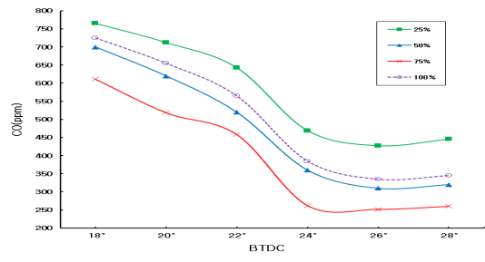
Figure 5. CO emission characteristics at various fuel injection timing
