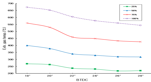
Figure 3. Exhaust gas temperature at various fuel injection timing
