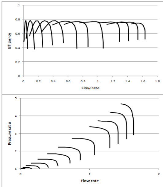
Fig. 4 Expanded Compressor Map
