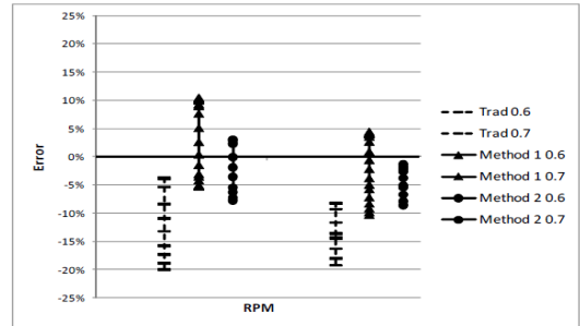
Fig. 1 Comparing Error Distributions
