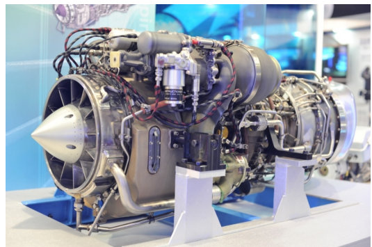
Fig. 2 T700/701K Engine
