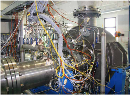
Fig. 6 Power Turbine Test Rig
