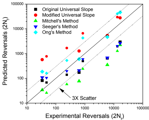
Fig. 1 Fatigue Life Prediction with Various Prediction Methods
