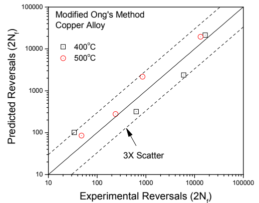
Fig. 2 Fatigue Life Prediction of Copper Alloy with Modified Ong's Method
