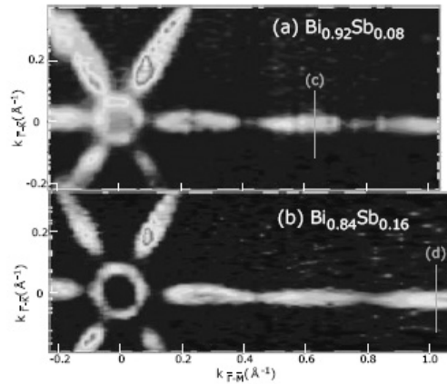
Fig. 1. The Fermi surface mapped by ARPES at 10 K for 40 Å thick Bi 0.92 Sb 0.08 (a) and Bi 0.84 Sb 0.16 (b) films, respectively. A circularly polarized light was used at the photon energy of 28 eV.
