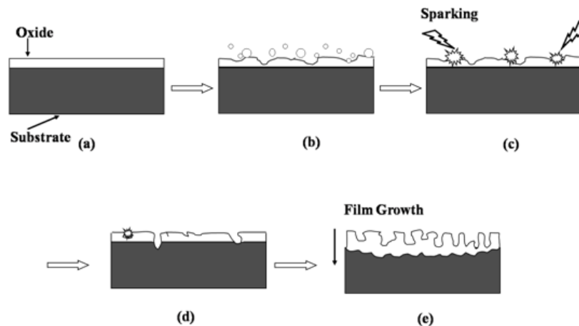
Fig. 1. The Schematic diagram of TiO 2 film formation
