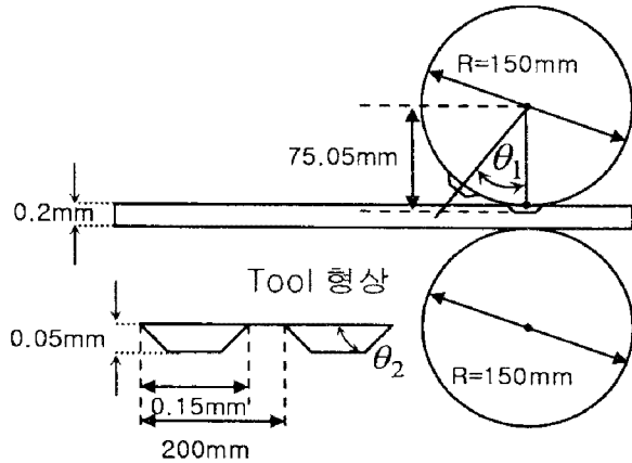
Fig. 1 Configuration of the analysis model
