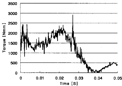
Fig. 5 Predicted forming torque
