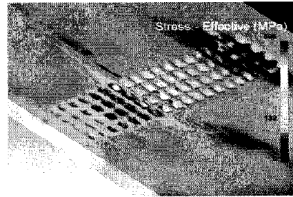
(c) After 2.28° rotation of the roll
