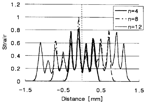
Fig. 9 Predicted effective strain distributions along the section AB for the various pattern numbers.
