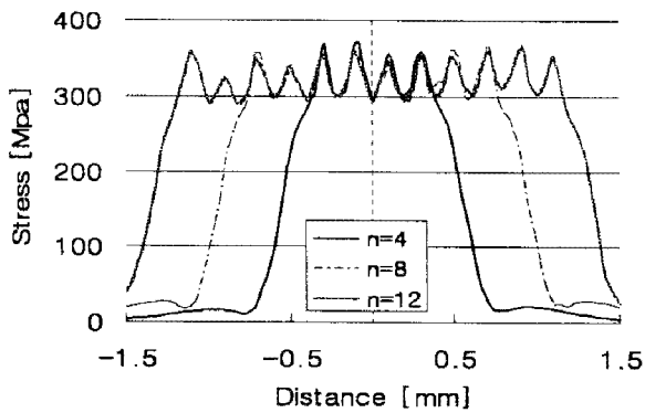
Fig. 8 Predicted effective stress distributions along the section AB for the various pattern numbers.
