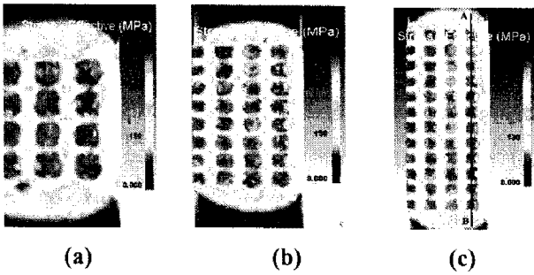
Fig. 7 Effective stress distribution on the sheet for the number of patterns of (a) 4, (b) 8, and (c) 12
