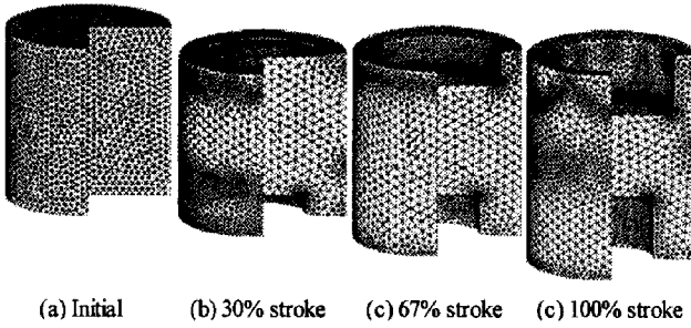
Fig. 2 History of plastic deformation
