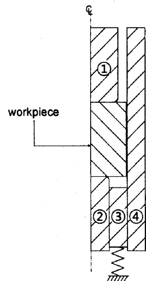
Fig. 1 Test axisymmetric back pressure forging process
