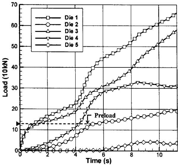
Fig. 6 Forming load variation with time
