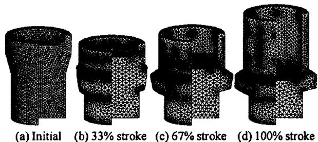
Fig. 5 History of plastic deformation
