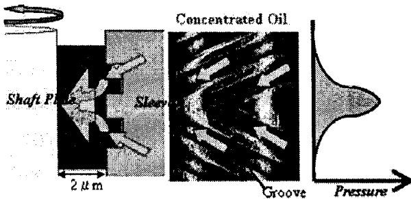
Fig. 2 Radial groove shape and pressure profile
