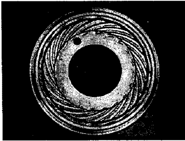
No. of groove : 20 ea., angle : 20°, depth : 15μm Fig. 1 Thrust groove shape and specification
