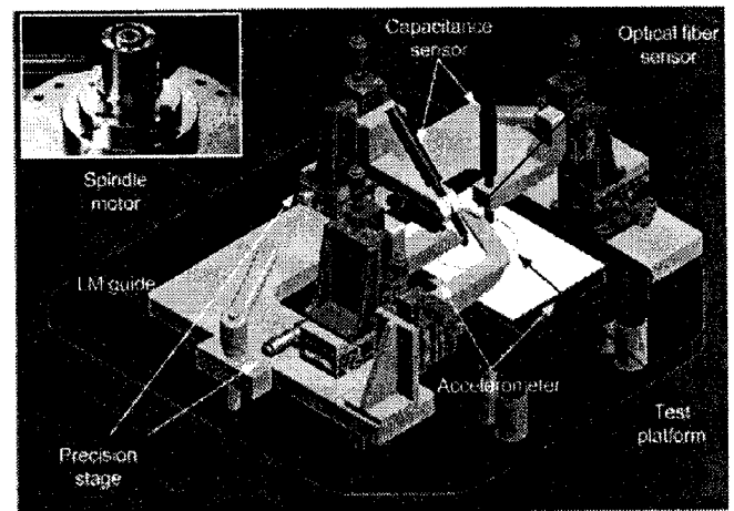
Fig. 4 Developed system for measuring dynamic characteristics of spindle motor assembly
