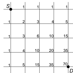
Fig. 2: The number of shortest paths from any node in the network to reference node S
