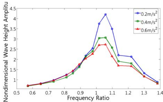
Fig. 7 Transfer functions from shaking table acceleration with various amplitudes to liquid displacement
