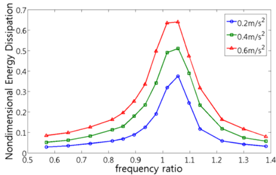
Fig. 10 Dissipation energy per a cycle with various excitation amplitudes
