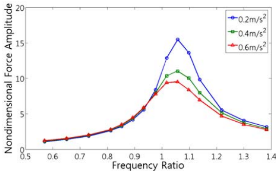
Fig. 9 Transfer functions from shaking table acceleration with various amplitudes to control force
