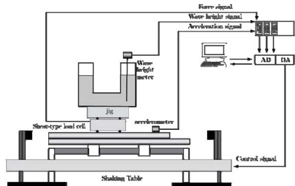
Fig. 5 Outline of shaking table test
