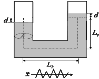
Fig.1 TLCD subjected to input acceleration
