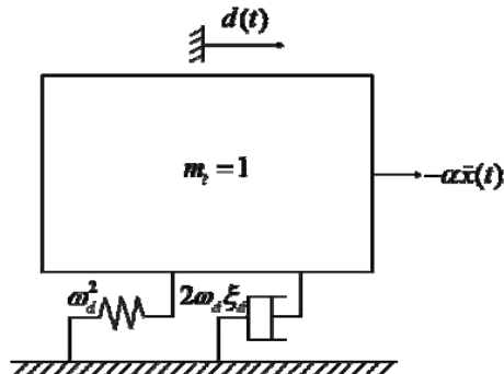
Fig. 2 Equivalent TMD model of a TLCD
