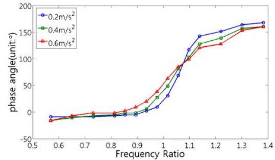
Fig. 8 Phase angles between shaking table accelerations with various amplitudes and liquid displacement
