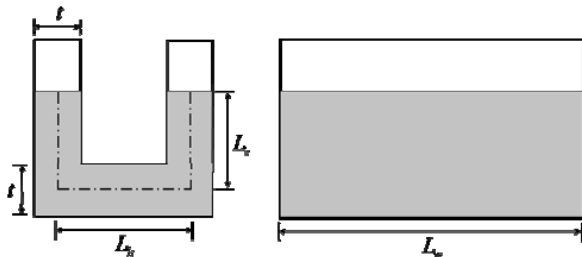
Fig. 3 Shape of TLCD specimen
