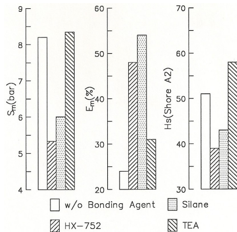
Fig. 3. Effect of Bonding Agents
