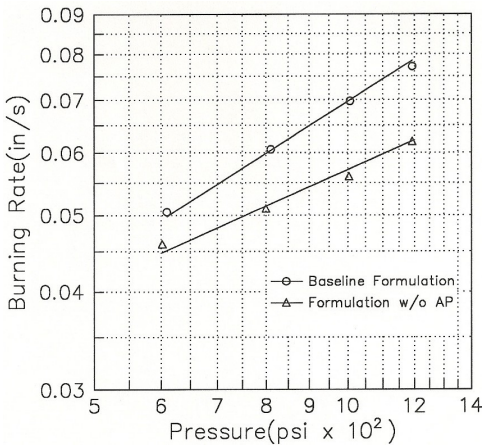
Fig. 4. Propellant Burning Rates Obtained from Strand Burner Tests
