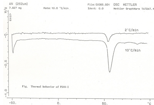
Fig. 1. DSC Thermograms of PSAN (AN-ZnO, 262 μ)
