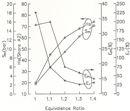
Fig. 2. Effect of Curative Ratio on Mechanical Properties of HTPB/AN Propellant
